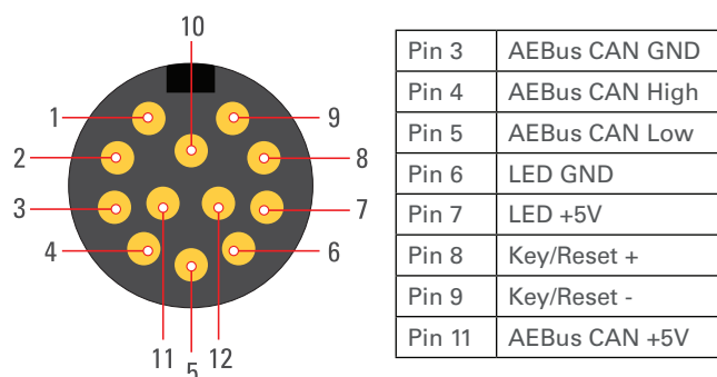
Circular 12 PIN (12-36-6700)
