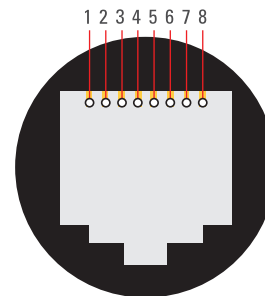
RJ45 AEBus (42-48-6650)
